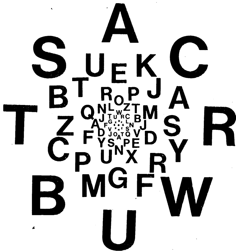
Fig. 4. Same dimensions as Fig. 3, but with more letters. Increasing the number of letters makes each letter harder to read, owing to supramacular masking effects, not owing to acuity limitations. However, all letters can be correctly read off an afterimage.
